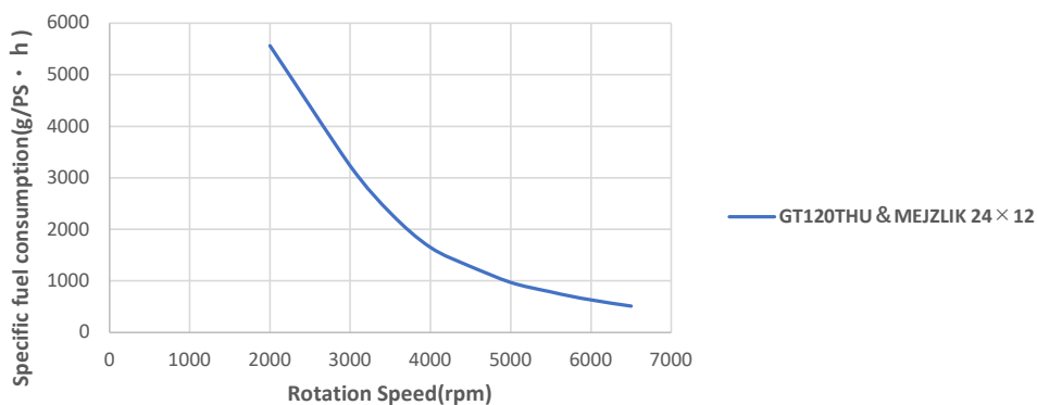
Specific fuel consumption (GT120THU)
