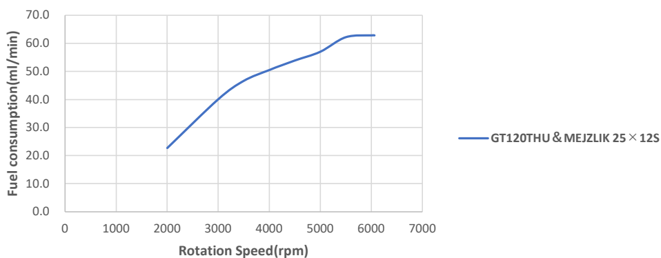
Fuel consumption(GT120THU)
