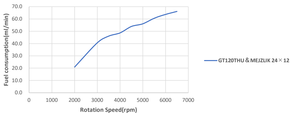
Fuel consumption (GT120THU)
