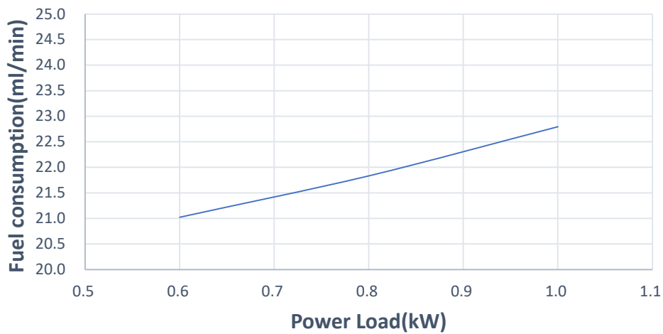
Fuel consumption(GT33REU)
