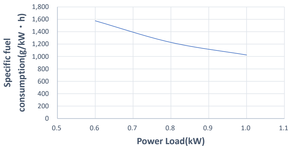
Specific fuel consumption(GT33REU)
