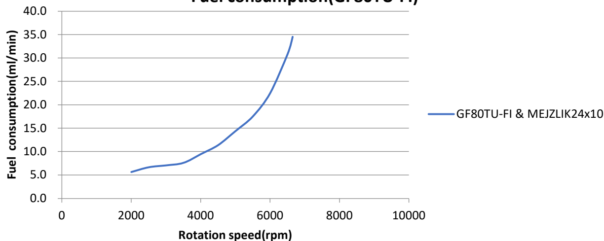
Fuel consumption(GF80TU-FI)
