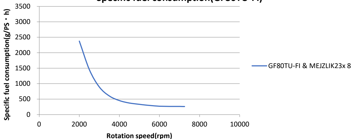
Specific fuel consumption(GF80TU-FI)
