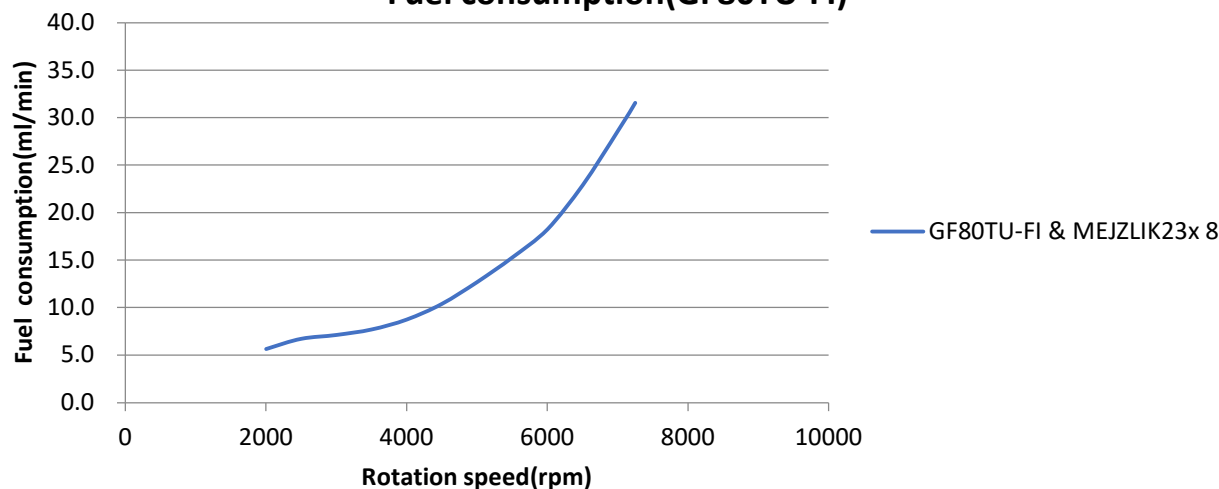
Fuel consumption(GF80TU-FI)
