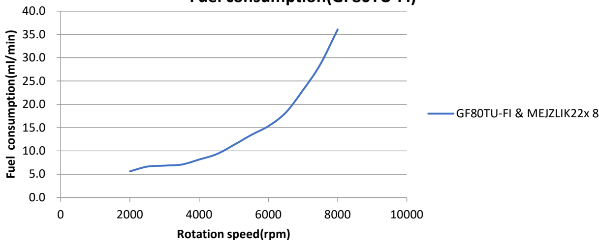
Fuel consumption(GF80TU-FI)
